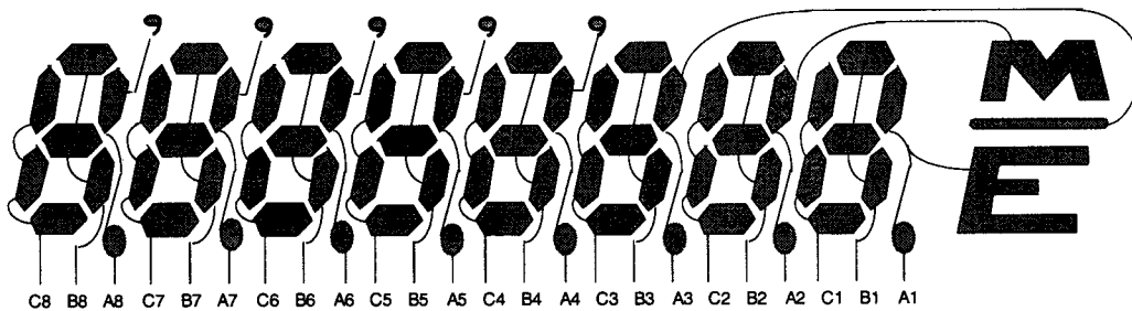
Segment Connection
